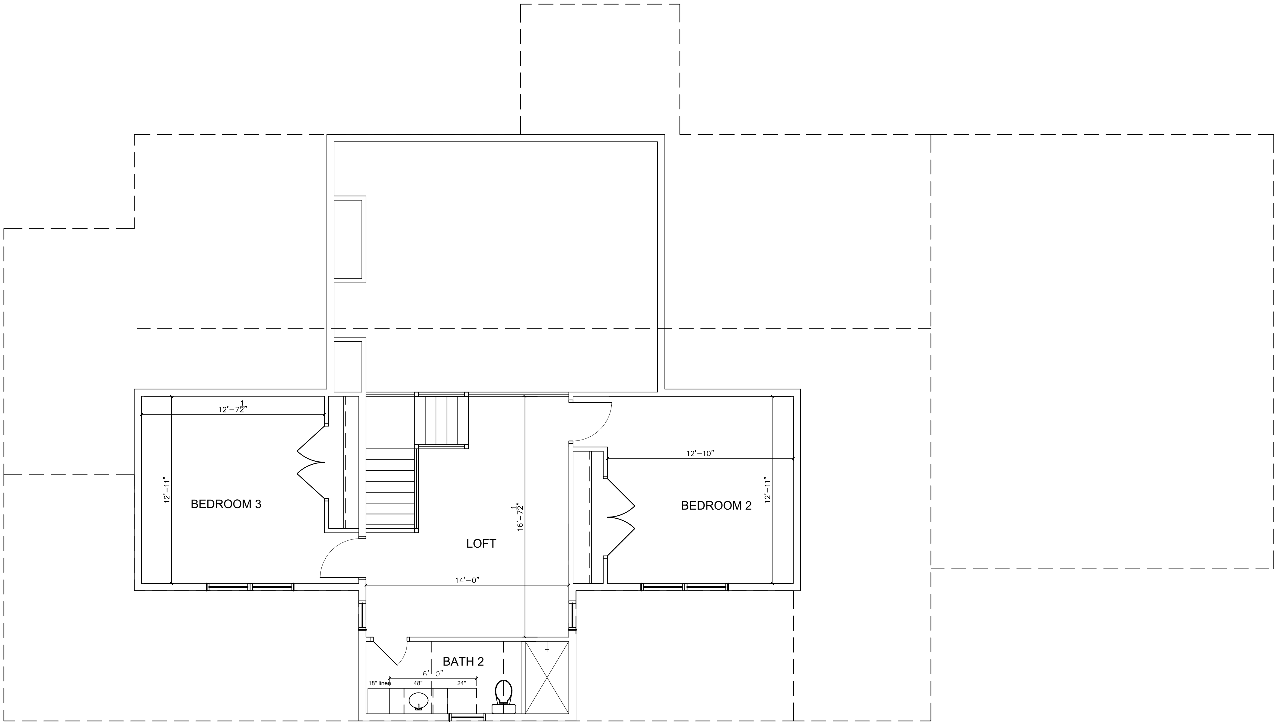
1 A-4 SECOND FLOOR PLAN 1/4" = 1'-0"
